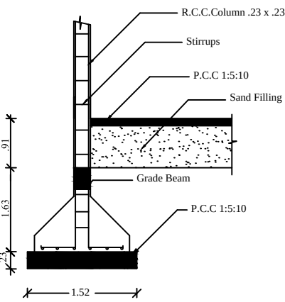
COLUMN DETAIL
