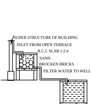
RAINWATER HARVESTING
