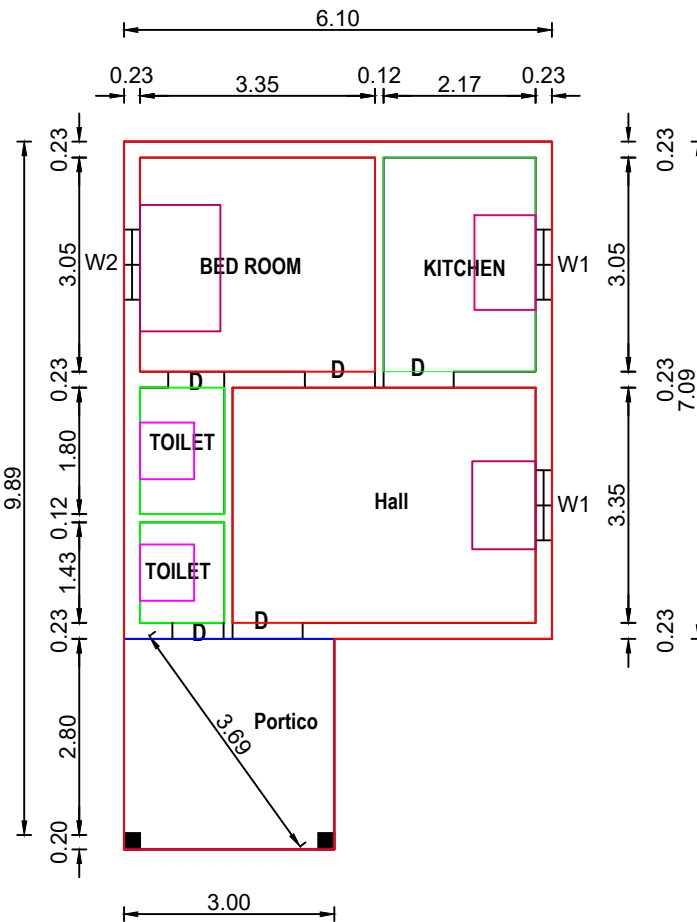
GROND FLOOR PLAN
