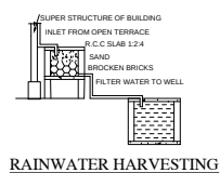
RAINWATER HARVESTING
