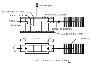
PLUMBING LAYOUT
