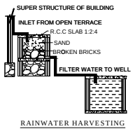
RAINWATER HARVESTING
