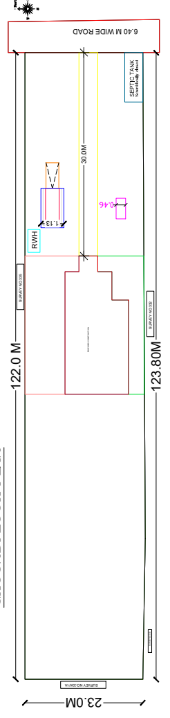
GROUND FLOOR PLAN
