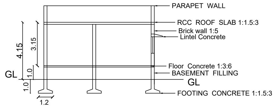
SECTION A-A VIEW
