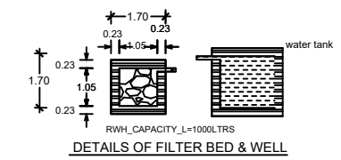
DETAILS OF FILTER BED & WELL
