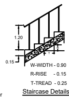
Staircase Details
