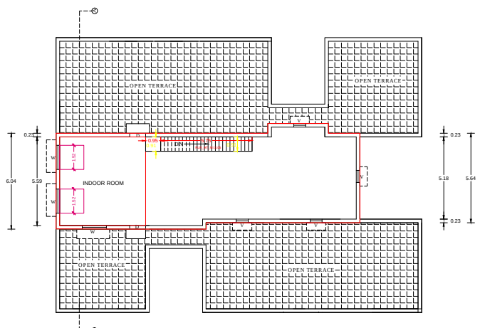
PRO. FIRST FLOOR PLAN
