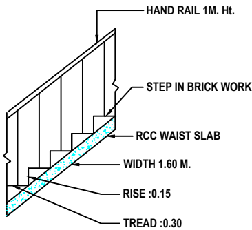
STAIR DETAIL
