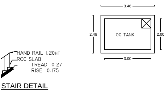
STAIR DETAIL
