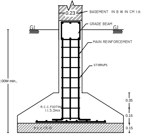
COLUMN DETAILS
