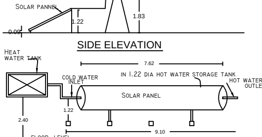
SOLAR WATER HEATER PLANT
