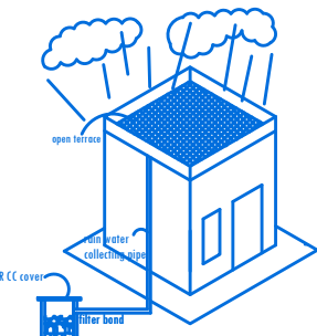
RAIN WATER HARVESTING ARRANGEMENT
