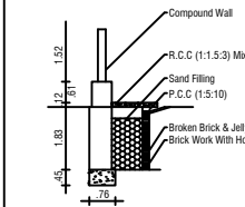
RAIN WATER HARVEST DETAILS
