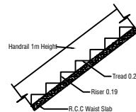
STAIR DETAILS
