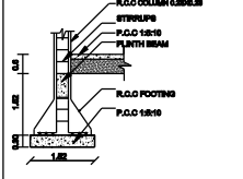
COLUMN DETAILS
