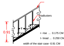
Details of staircase
