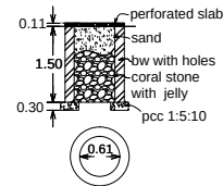
percolation pit
