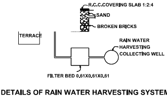
DETAILS OF RAIN WATER HARVESTING SYSTEM
