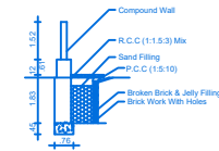
RAIN WATER HARVEST DETAILS
