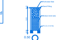
RAIN WATER COLLECTION WELL
