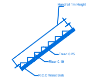
STAIR DETAILS
