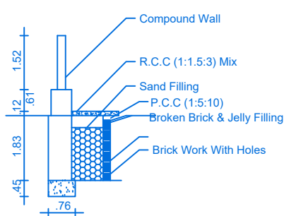
RAIN WATER HARVEST DETAILS
