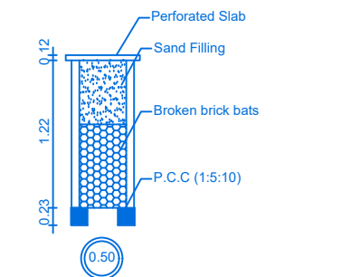
RAIN WATER COLLECTION WELL
