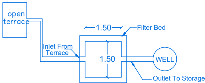
Plan Of Filter Bed & Well
