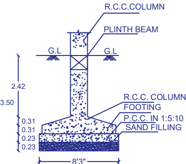
FOUNDATION DETAIL (DETAIL - B)
