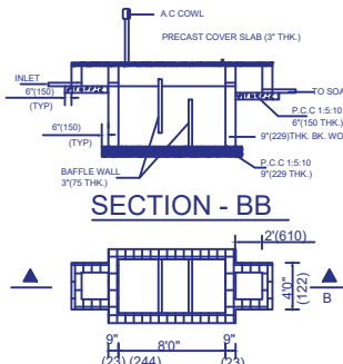
PLAN OF SEPTIC TANK
