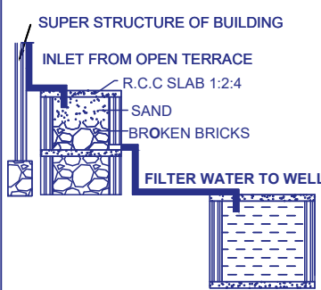
RAINWATER HARVESTING
