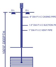
BORE WELL
