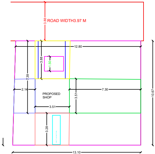
SITE PLAN
