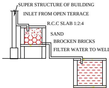
RAINWATER HARVESTING
