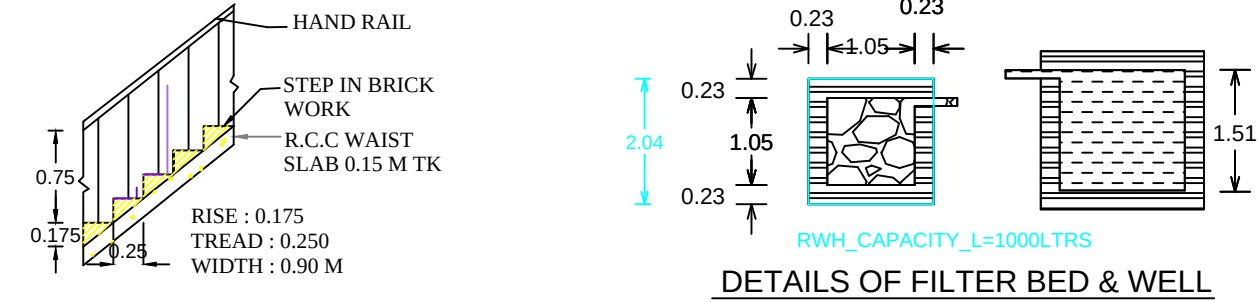
STAIR DETAILS
