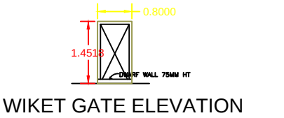
WIKET GATE ELEVATION
