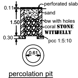
percolation pit
