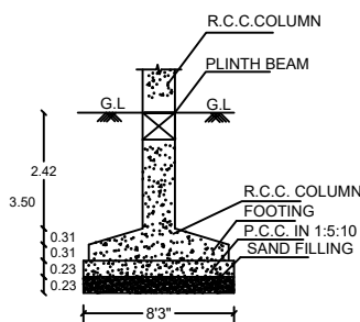
FOUNDATION DETAIL
