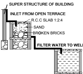
RAINWATER HARVESTING
