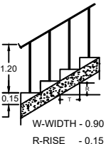
Staircase Details
