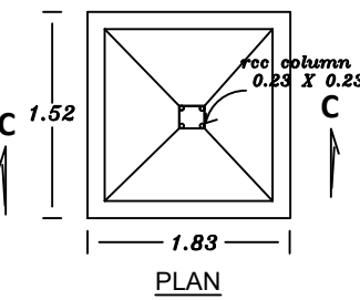
Details of coloumn footing
