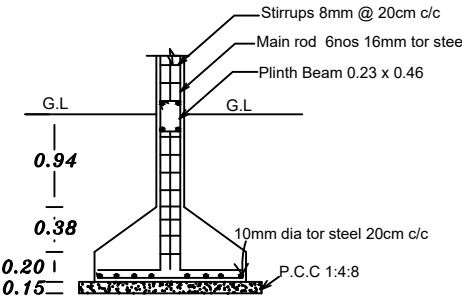
Details of coloumn footing
