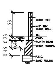
COMPOUND WALL DETAILS - N.T.S
