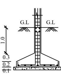
COLUMN FOOTING DETAILS - N.T.S
