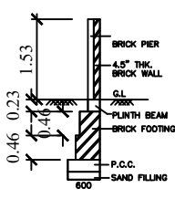
COMPOUND WALL DETAILS - N.T.S
