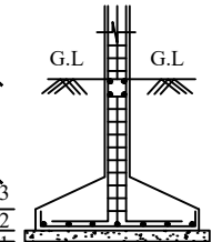
COLUMN FOOTING DETAILS - N.T.S
