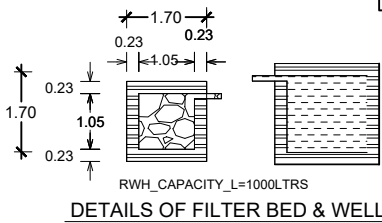
DETAILS OF FILTER BED & WELL
