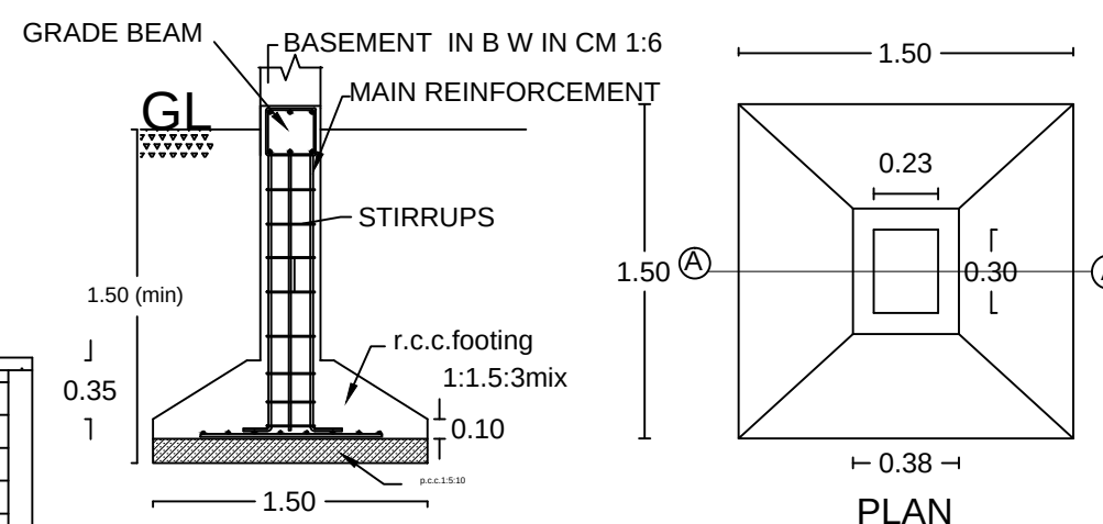
COLUMN DETAILS
