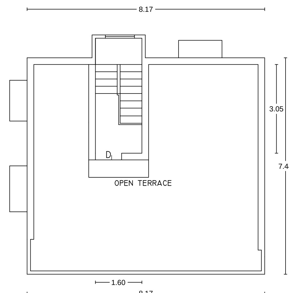
HEAD ROOM FLOOR PLAN
