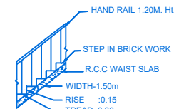
STAIR DETAIL
