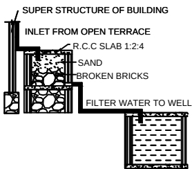
RAINWATER HARVESTING
