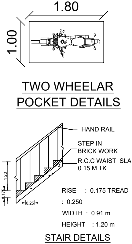
STAIR DETAILS
