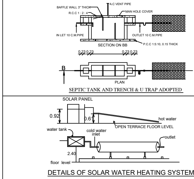
DETAILS OF SOLAR WATER HEATING SYSTEM
