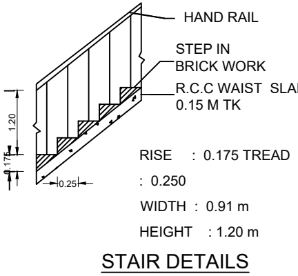
STAIR DETAILS
