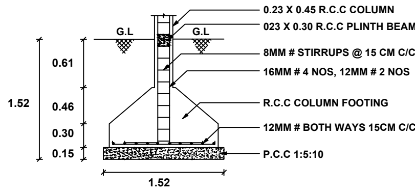
COLUMN FOOTING DETAILS
