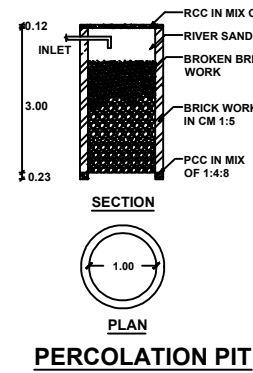
PERCOLATION PIT
