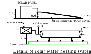
Details of solar water heating system
