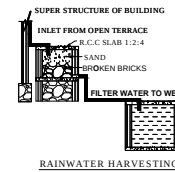
RAINWATER HARVESTING
