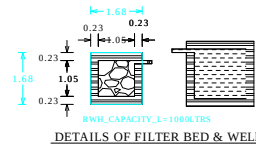
DETAILS OF FILTER BED & WELL
