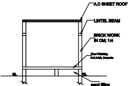
SECTION NN
