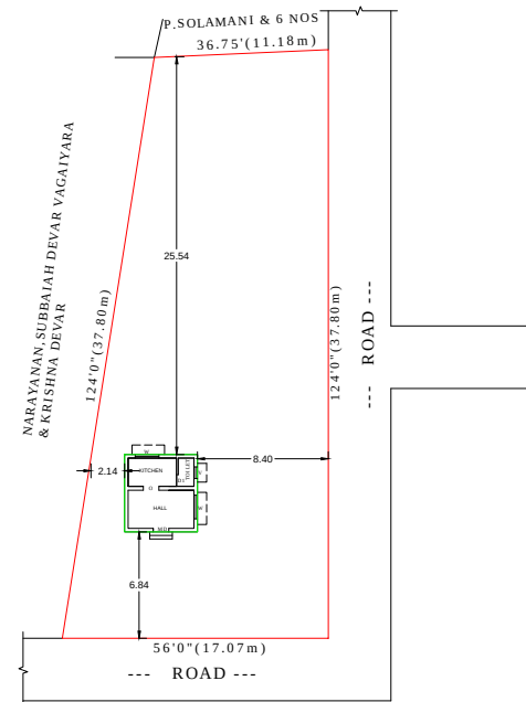
SITE PLAN
