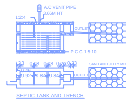
SEPTIC TANK AND TRENCH
