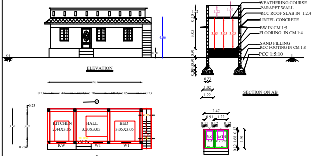
PLAN OF BATH & TOILET
