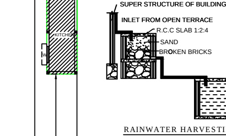
RAINWATER HARVESTING
