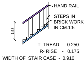
DETAILS OF STAIRCASE
