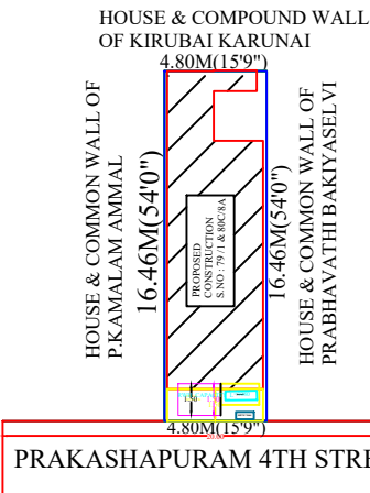
SITE PLAN
