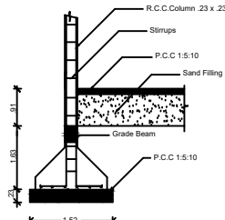
COLUMN DETAIL
