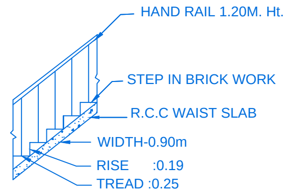
STAIR DETAIL
