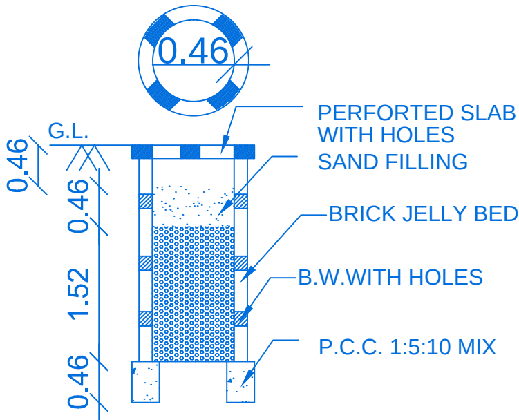
PERCOLATION PIT
