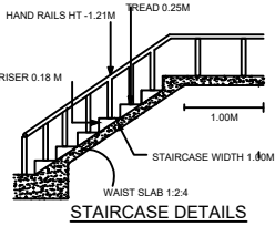
STAIRCASE DETAILS
