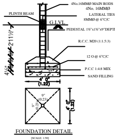
FOUNDATION DETAIL (SCALE: 1/10)
