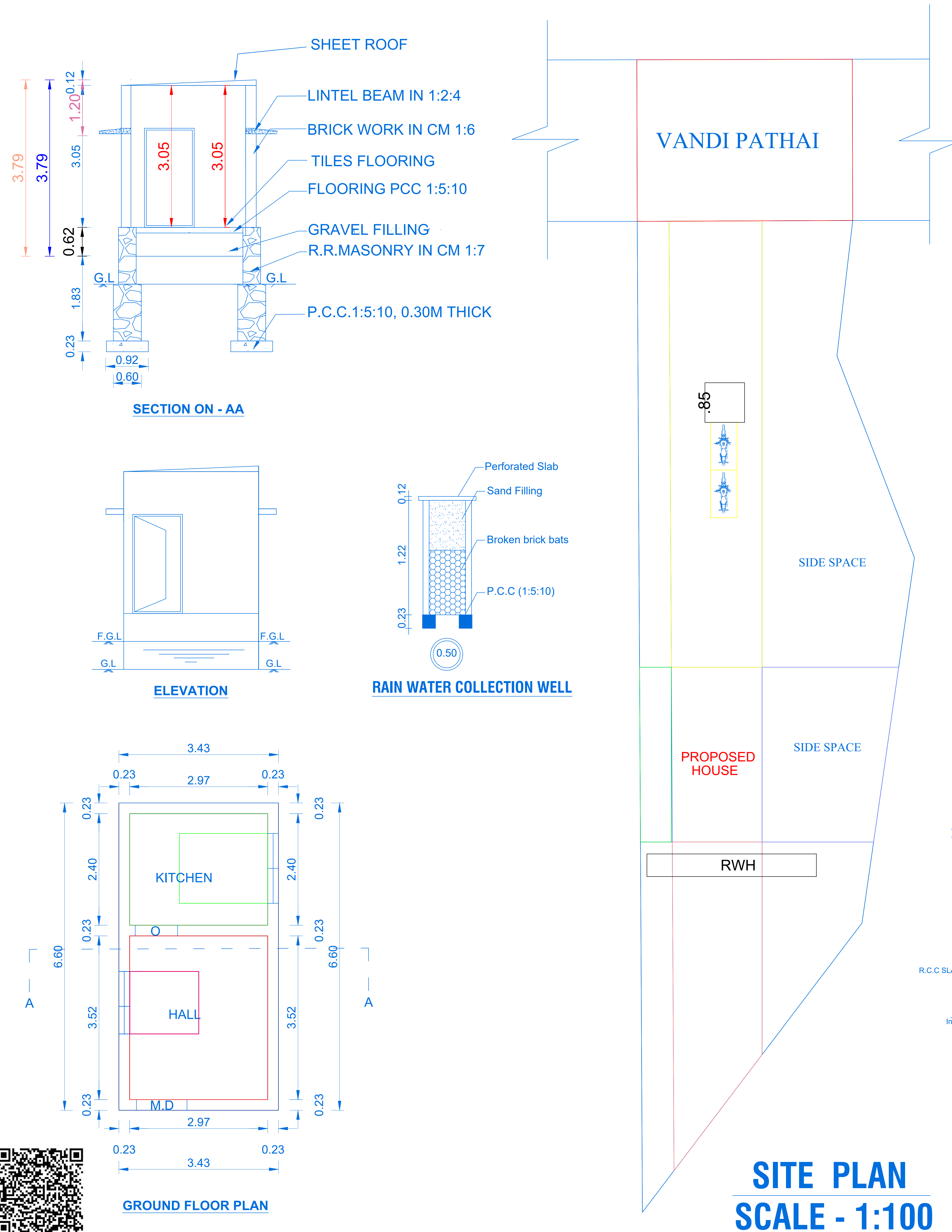
RAIN WATER HARVEST DETAILS
