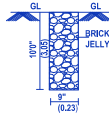
PERCOLATION PIT
