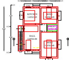
PRO.GROUND FLOOR PLAN
