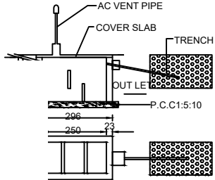
SEPTIC TANK
