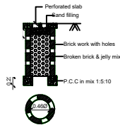
PERCOLATION PIT FOR 30 Sq. m. (Scale:- 1:50)
