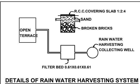
DETAILS OF RAIN WATER HARVESTING SYSTEM
