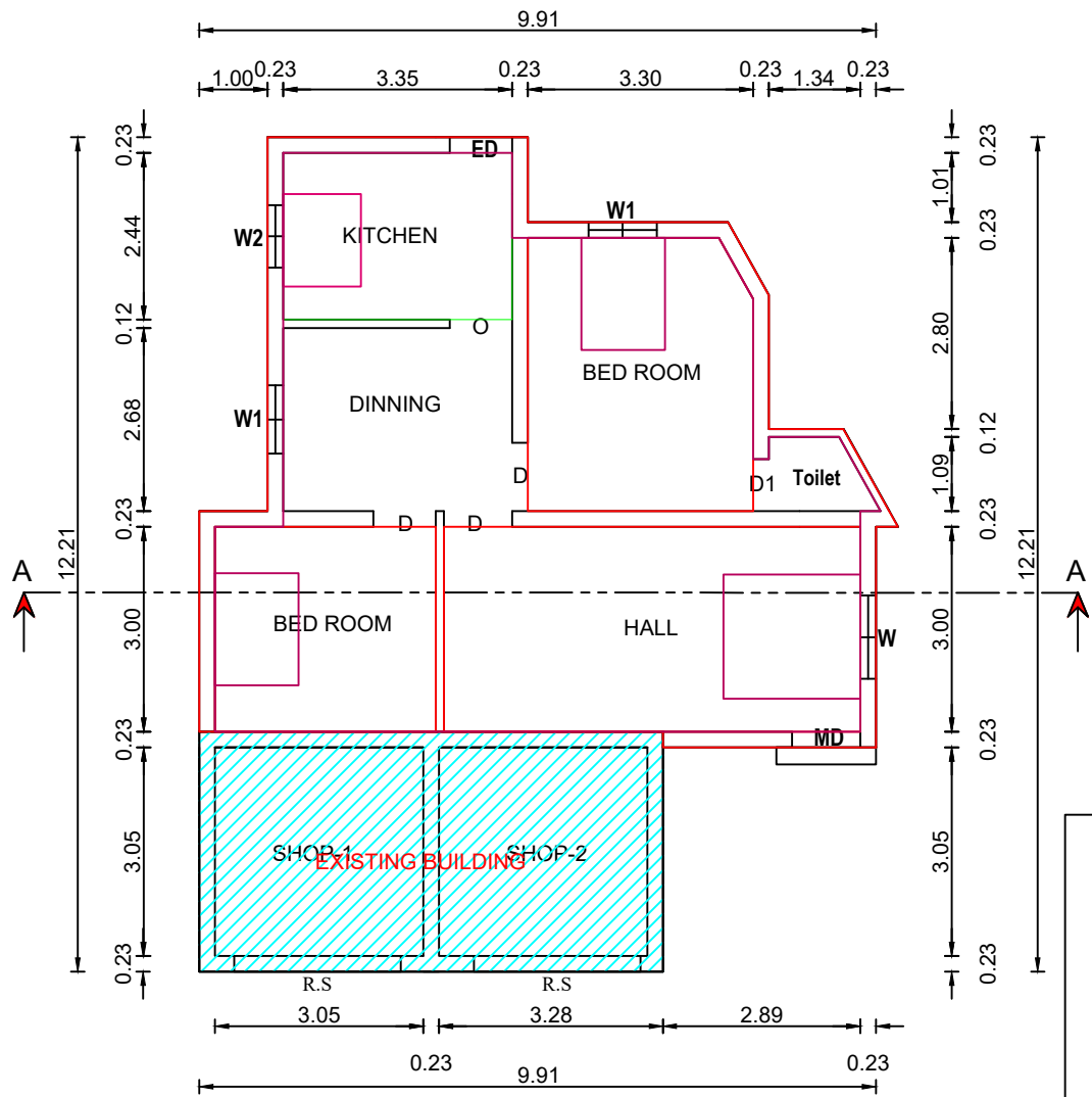
GROND FLOOR PLAN
