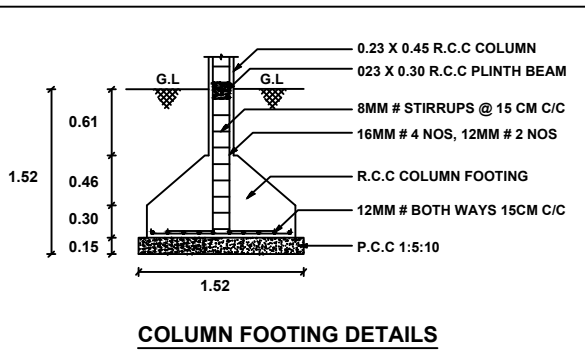
COLUMN FOOTING DETAILS
