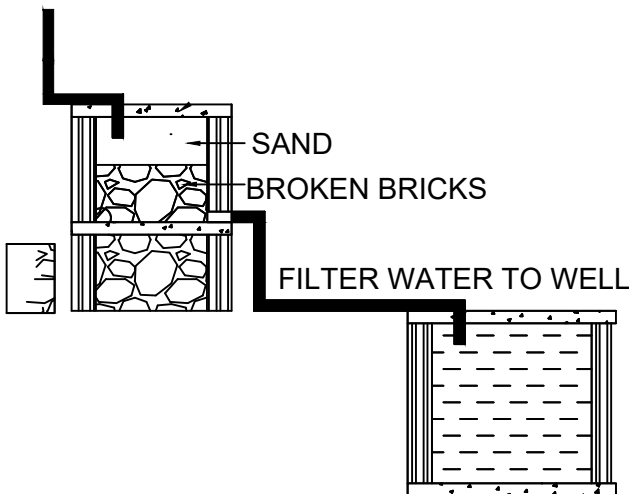
RAINWATER HARVESTING
