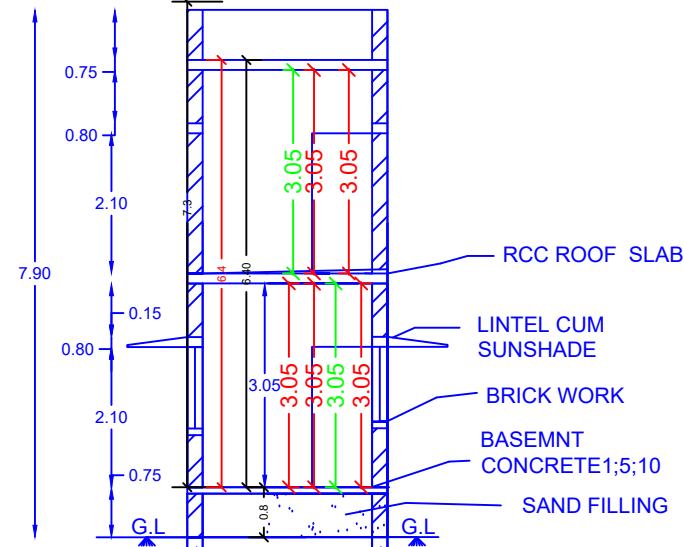
SECTION AB
