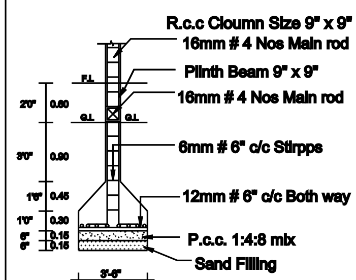
COLUMN DETIAL
