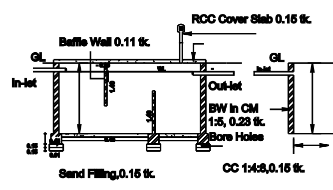
SEPTIC TANK & SOAK PIT
