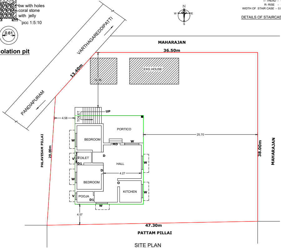
SITE PLAN
