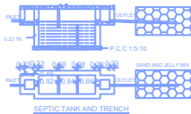
SEPTIC TANK AND TRENCH
