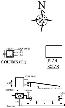
Details of solar water heating system
