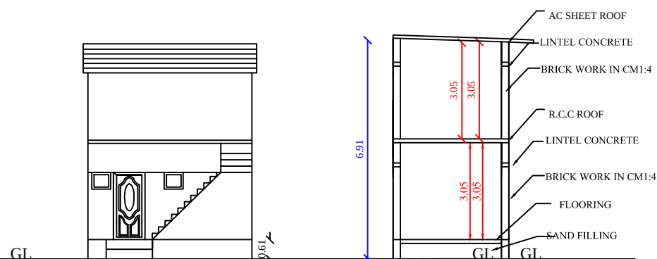
SECTION ON AB&CD
