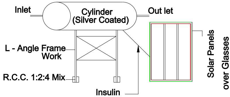
SOLAR ENERGY
