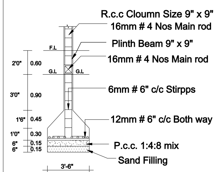
COLUMN DETIAL
