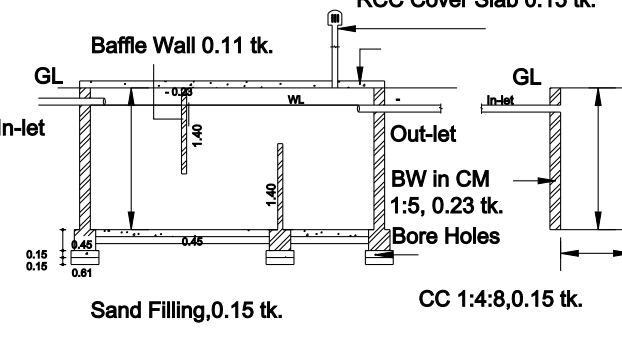
SEPTIC TANK & SOAK PIT
