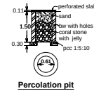
Percolation pit
