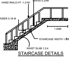
STAIRCASE DETAILS
