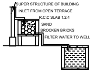
RAINWATER HARVESTING
